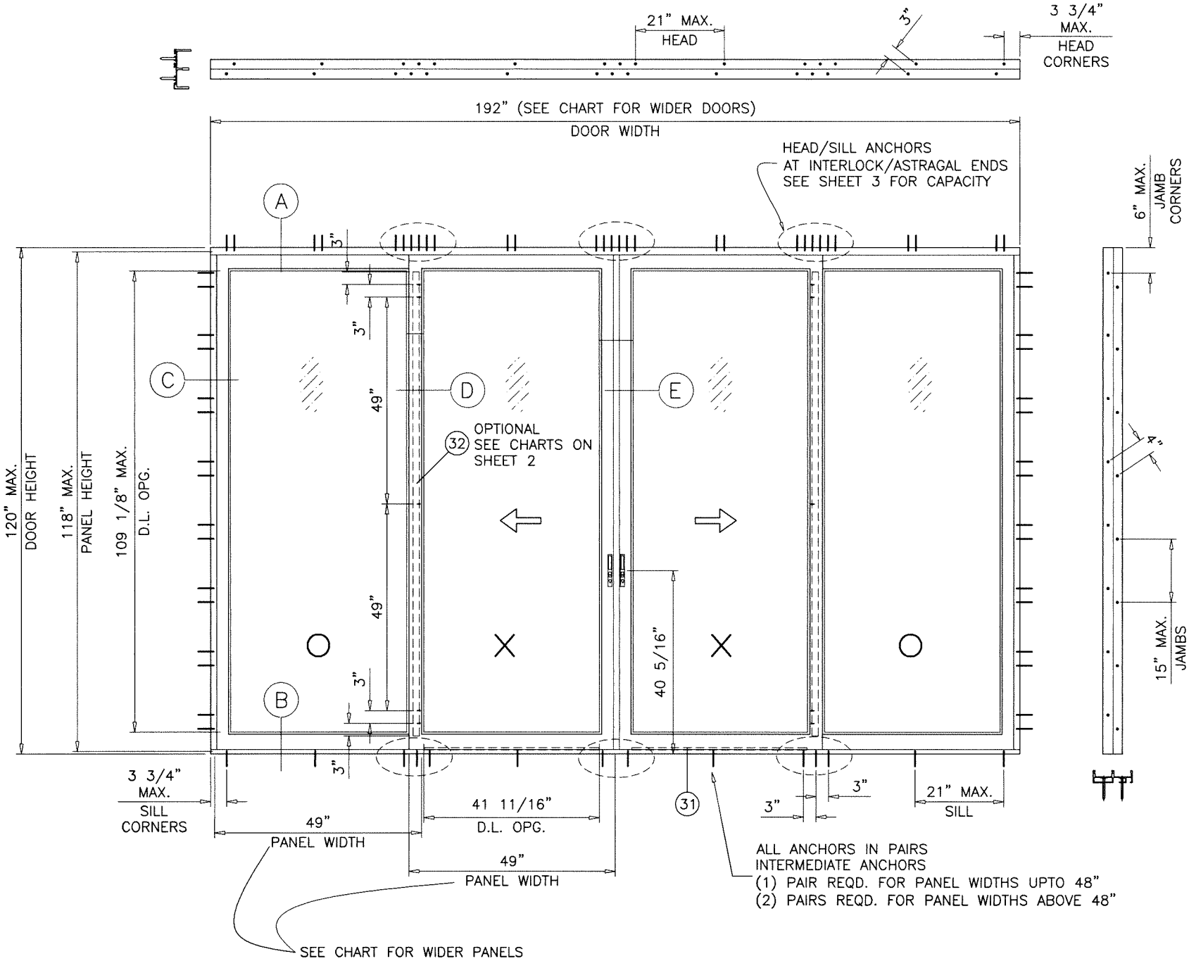
TYPICAL ELEVATION TESTED UNIT
